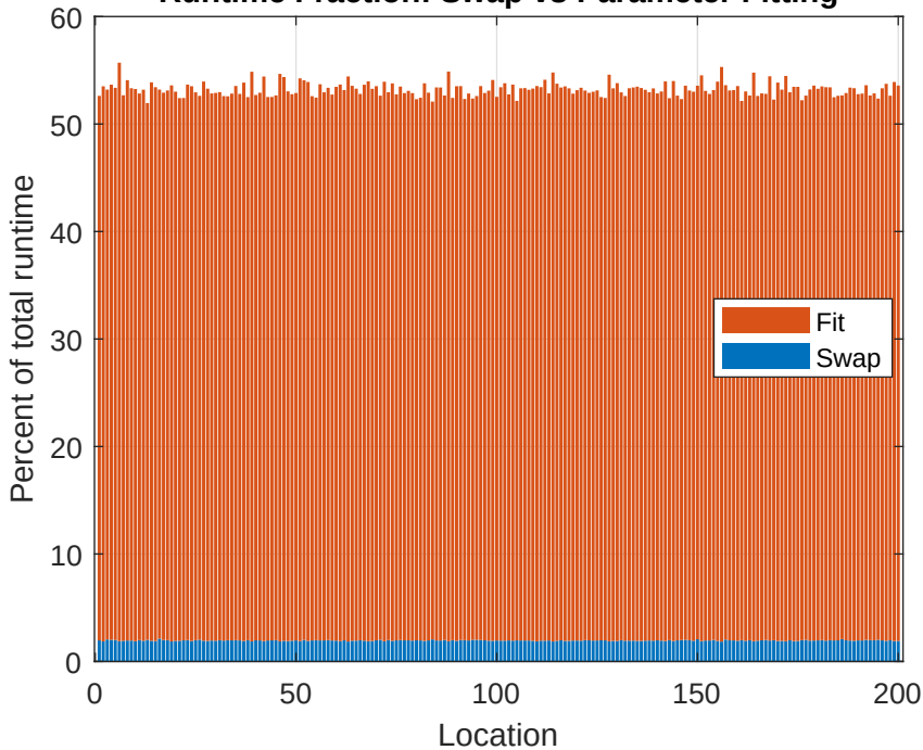
Runtime Fraction: Swap vs Parameter Fitting
